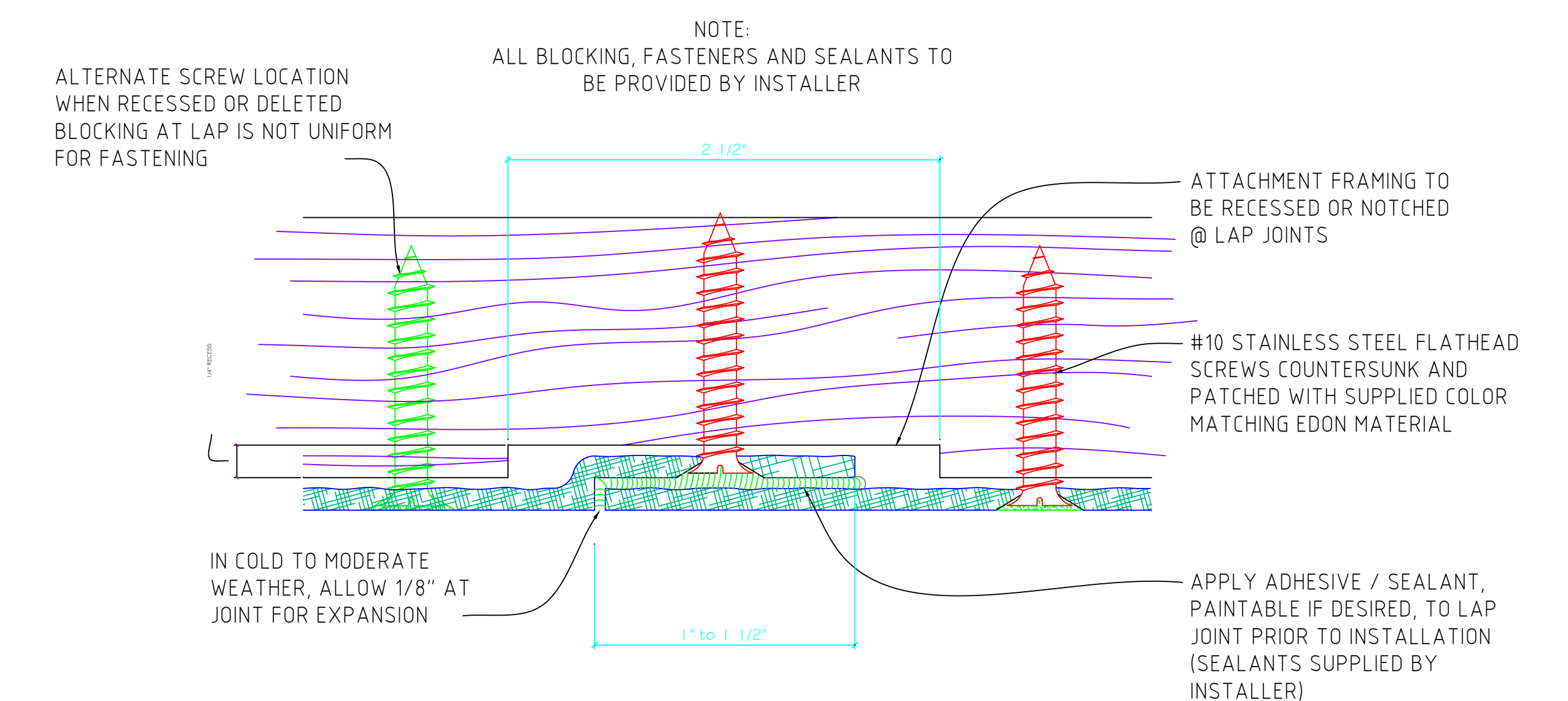
B LAP JOINT DETAIL 1 FULL SCALE
