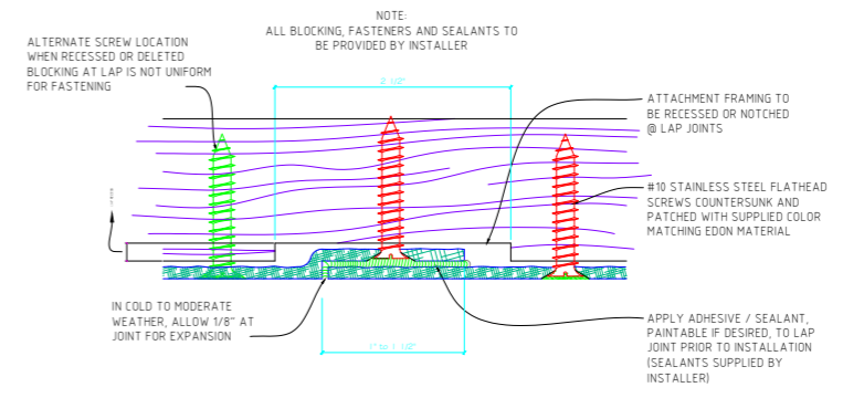
B LAP JOINT DETAIL 1 FULL SCALE
