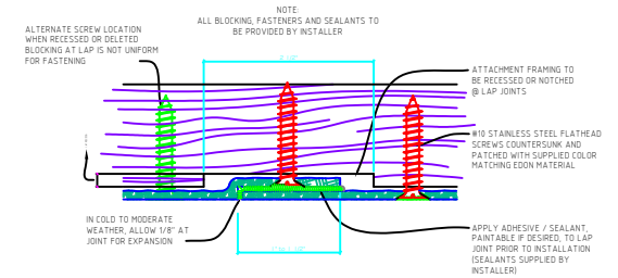
B LAP JOINT DETAIL 1 FULL SCALE
